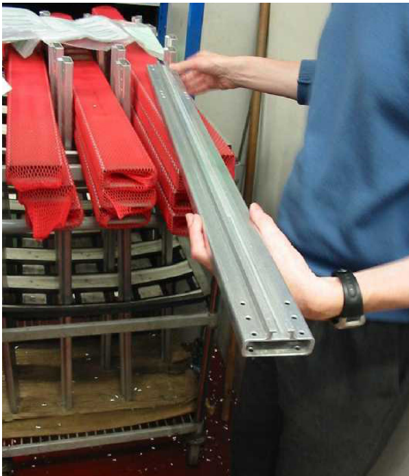
Ejection seat guide rails - wall thickness, gauged with the spindle probe is critical along the full length
