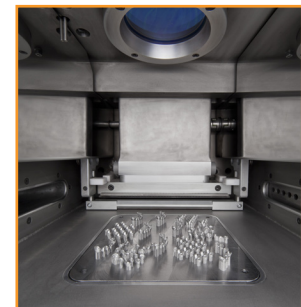
Laser melting machine build chamber
