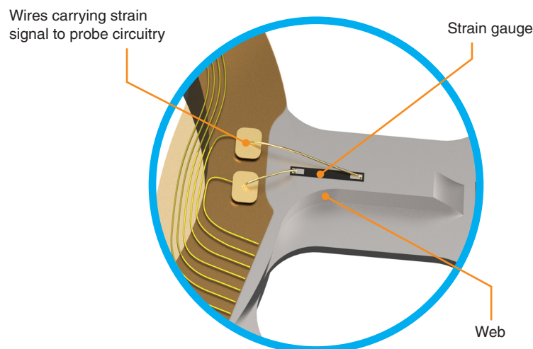
Figure 10: strain gauge mounted to web inside probe
