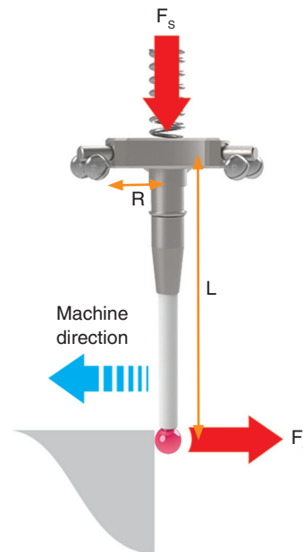
Figure 5: force balance in a touch-trigger- probe
