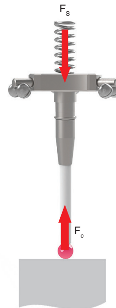
Figure 9: force balance in the Z direction
