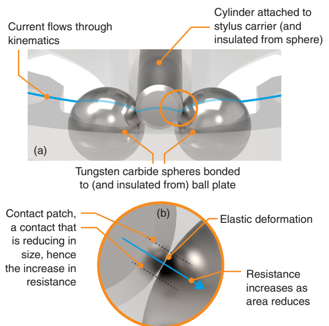
Figures 3a and 3b: (a) electrical circuit through kinematics and (b) close-up of the contact path between elements
