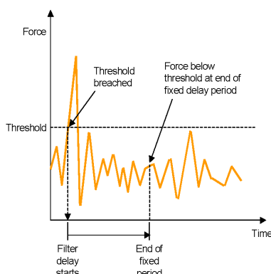
Figure 12a: a random vibration breaches strain gauge force threshold - no trigger issued
