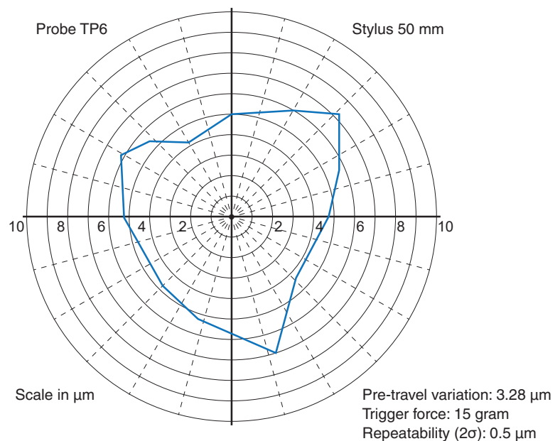
Figure 8: pre-travel variation plot for a TP6 CMM probe
