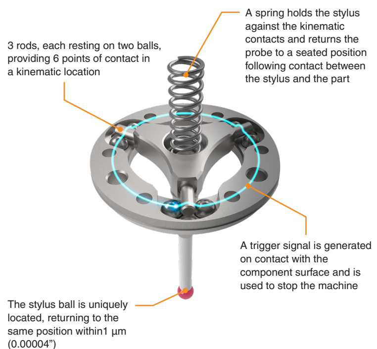
Figure 1: schematic of a kinematic resistive probe
