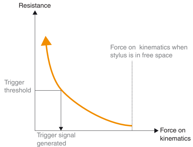
Figure 4: a trigger is generated when the probe circuit resistance breaches a threshold value
