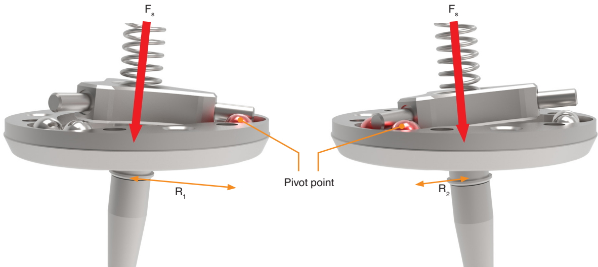
Figure 7a: pivot point is further from stylus centreline in high force direction
