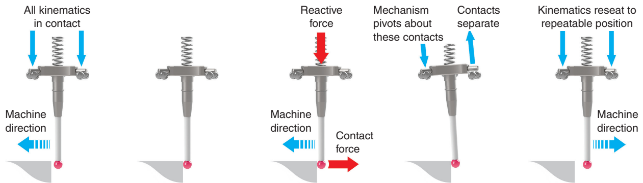
Figure 2: how a kinematic resistive probe generates a trigger
