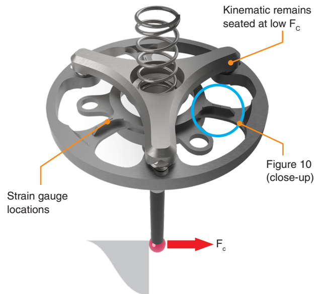
Figure 11: schematic of a strain gauge probe measuring the contact force
