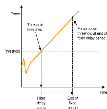
Figure 12b: a persistent force due to a probe trigger breaches strain gauge force - trigger signal is issued at the end of the delay period
