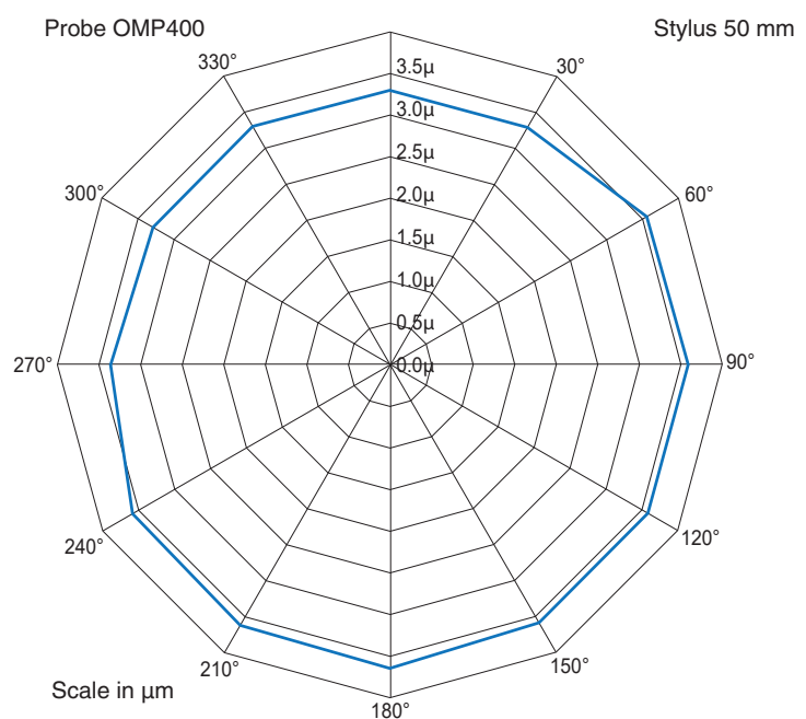
Figure 13: pre-travel variation plot for an OMP400 touch-trigger probe
