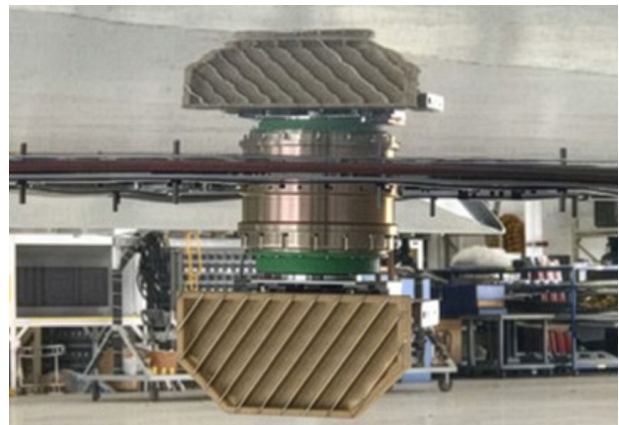
RF antenna and gimbal assembly on the belly of an aircraft
