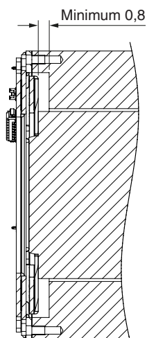
Section G-G
