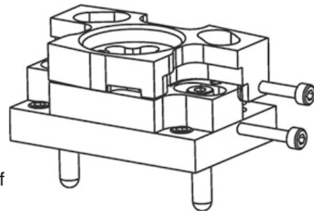
Figure 11 - 3-plate adjuster pack
