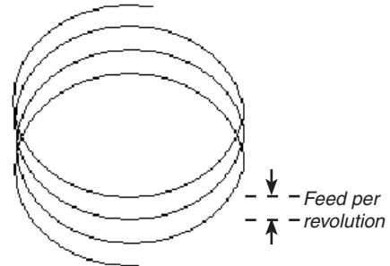
Figure 5b - Feed per revolution is a factor in diameter measurement uncertainty
