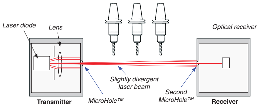
Figure 2 - Renishaw's transmitter unit features a lens that provides a narrow laser beam that passes through a small MicroHole™. The receiver further filters this light using a second MicroHole™, forming a very narrow, parallel measurement laser beam
