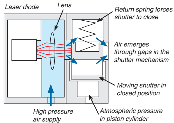
Figure 3a - During machining, conventional laser tool setters are protected by a moving shutter and continuous air 'bleed'
