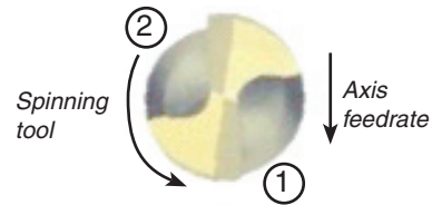
Figure 5a - One edge will extend further than the others from the centreline and will break the laser beam before the others
