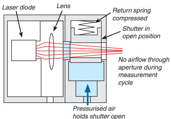
Figure 3c - Shutter is held open by pressurised air, whilst air bleed/blast is shut off to eliminate air turbulence along the laser beam
