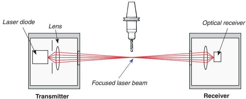
Figure 1 - Transmitter unit of a first generation laser tool setter providing a beam that is focused at a particular point between transmitter and receiver
