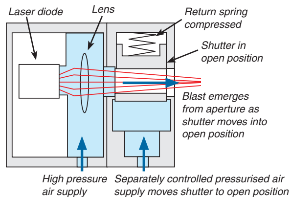
Figure 3b - Shutter is moved to open position by pressurised air, resulting in an air blast through the aperture as the trapped air in the optics chamber escapes
