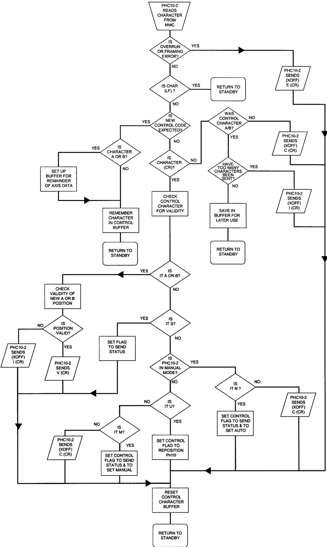
FLOWCHART 4 - RESPONSE OF PHC10-2 TO CHARACTERS TRANSMITTED BY MMC
