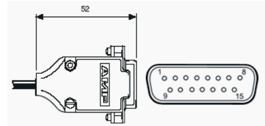
Figure 1 – Analogue quadrature input mating connector
