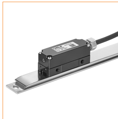
HiLin + HMS solid magnetic scale with welded cover foil
