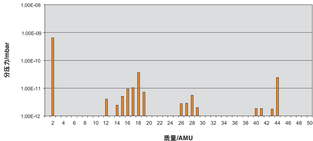
经过烘焙后的RESOLUTE UHV读数头 (带1.0 m电缆) (总压力 = 8 \times 10^{-10} \text{ mbar} )
