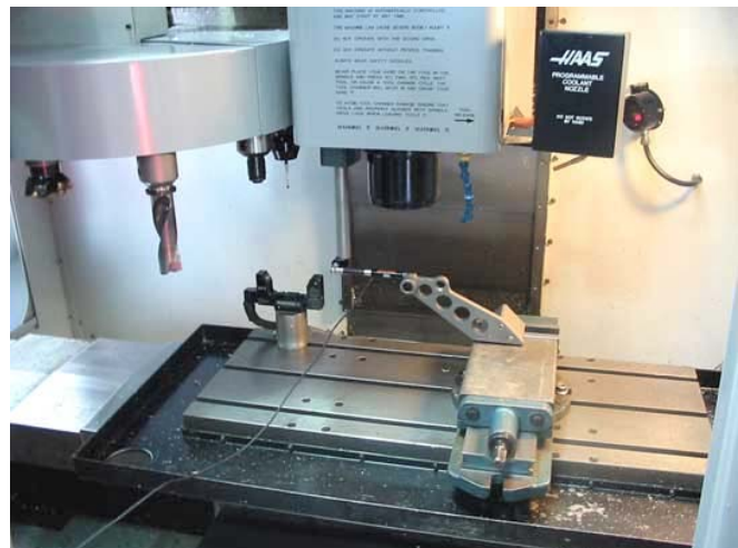
QC10 ballbar testing positioning performance on a HAAS VMC
